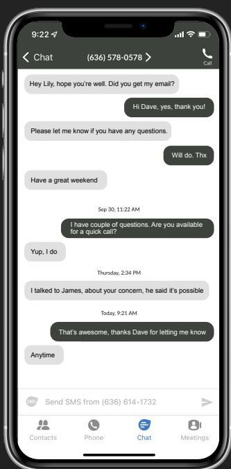
Mobile App
