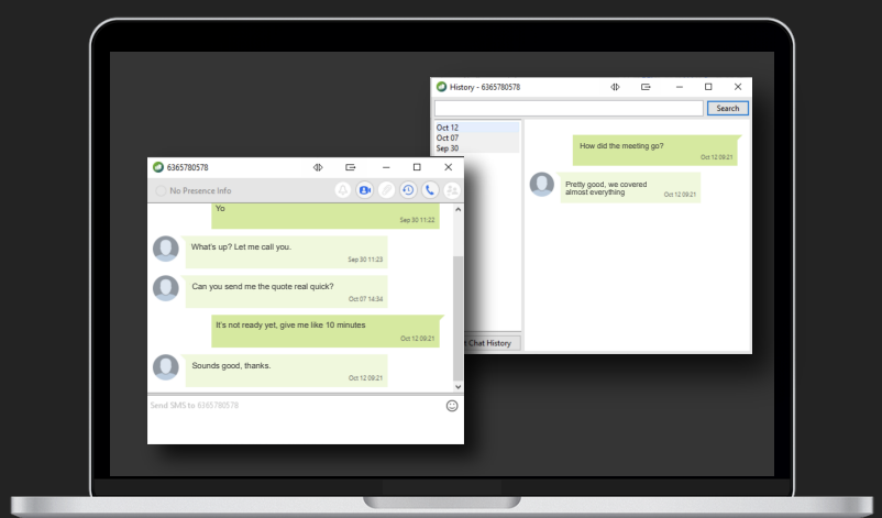
Desktop App
